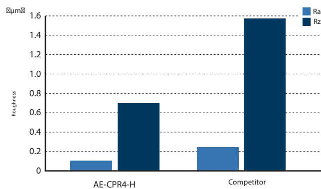
Bottom surface roughness after milling 80,2m
