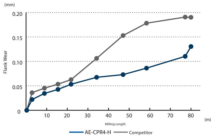
Wear comparison of the cutting edge after milling 80,2 m
