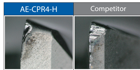
Wear comparison of the cutting edge after milling 80,2 m
